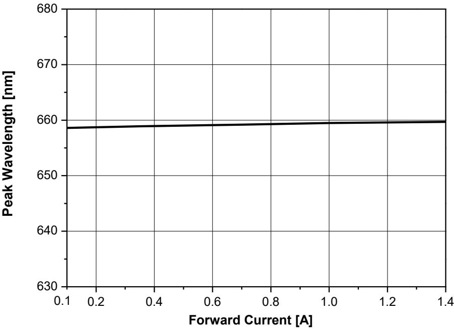
Fig 5. Forward Current vs Peak Wavelength, Tj=25°C
