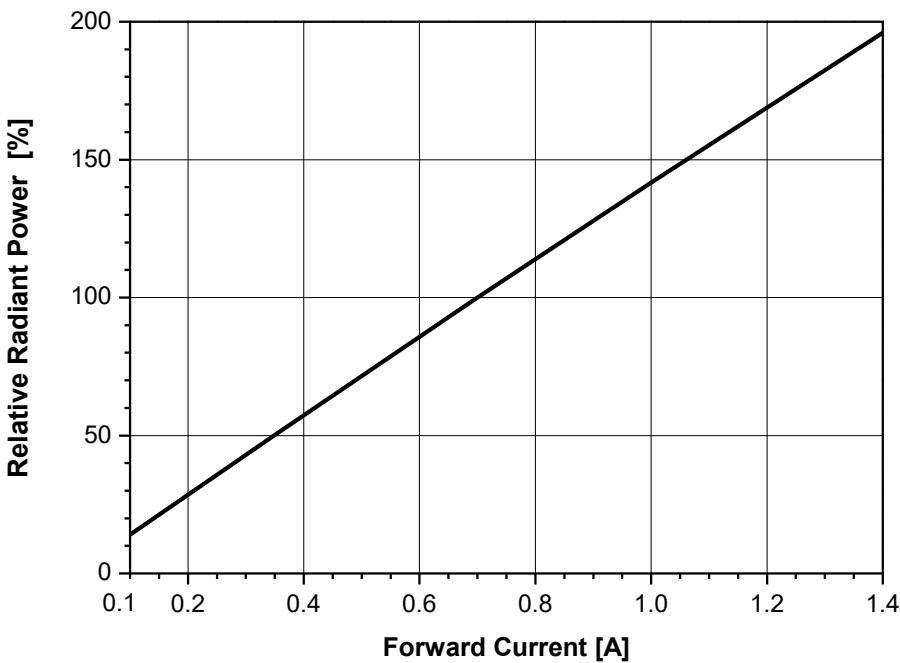
Fig 4. Forward Current vs. Normalized Relative Radiant Power, T_j=25^{\circ}\text{C}
