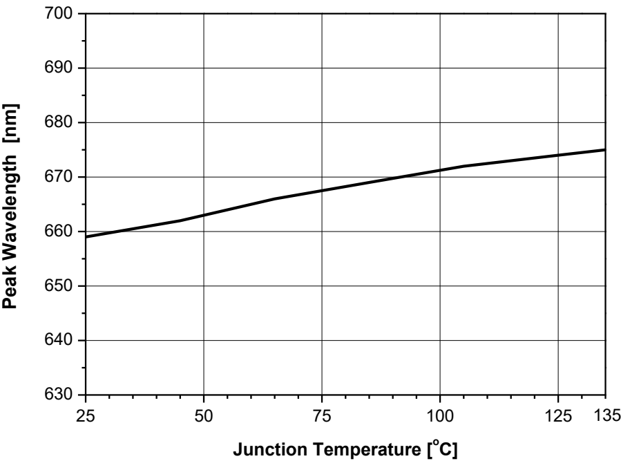
Fig 8. Junction Temperature vs. Peak Wavelength at IF=700mA
