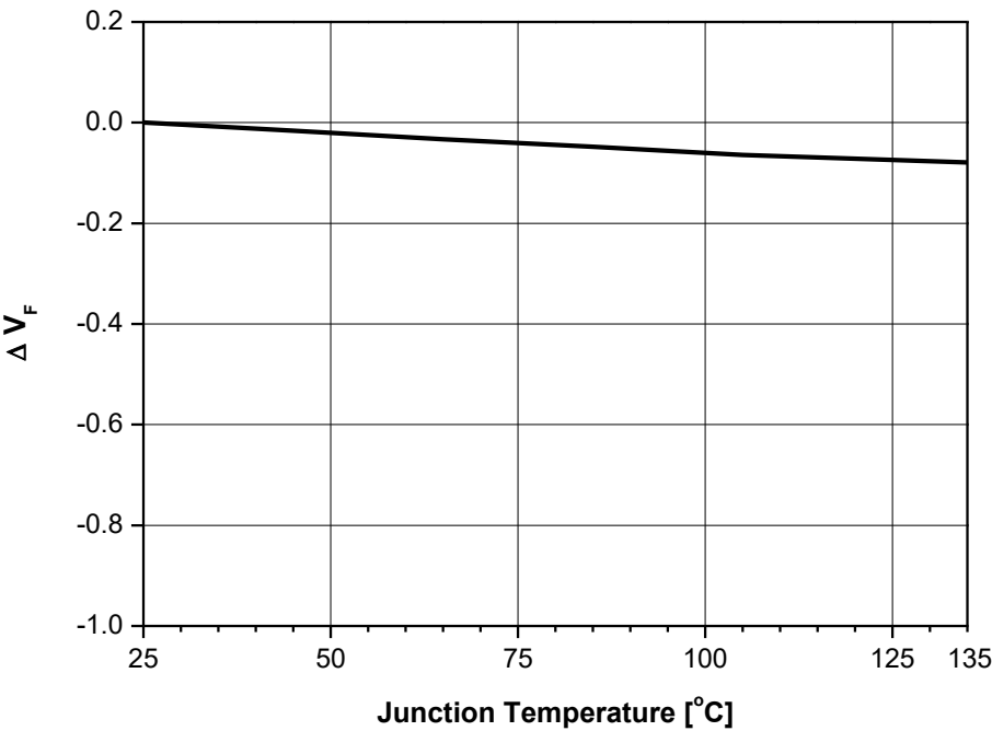
Fig 7. Junction Temperature vs. Forward Voltage at IF=700mA
